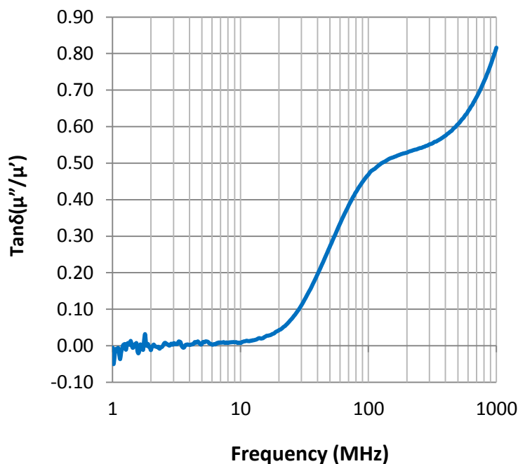
Magnetic Loss Tangent
